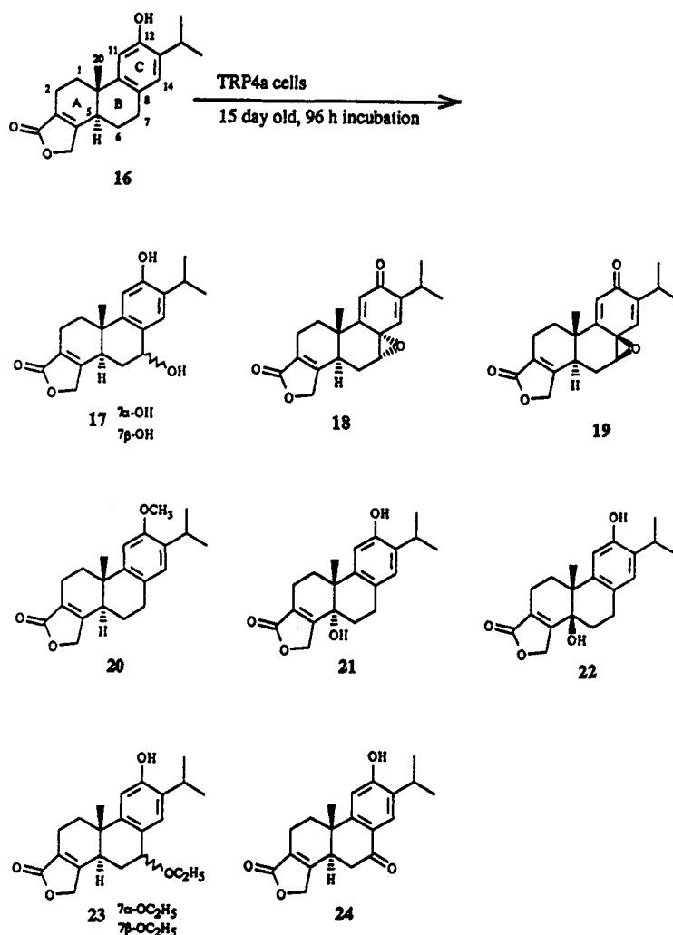
Fig. 3. Biotransformation of isotriptophenolide (16) with TRP4a cells.
