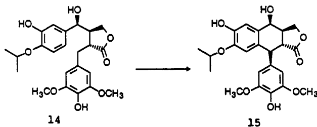
Fig. 2. Biotransformation of 14 to 15 with plant cell culture of P. peltatum (semi-continuous process) or with broth from cell culture of Nicotiana glauca .
