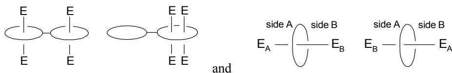
“Type 1 Isomerism”
